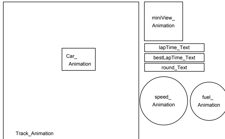
Fig. 5. Example user interface presentation for the scene RacingScene
