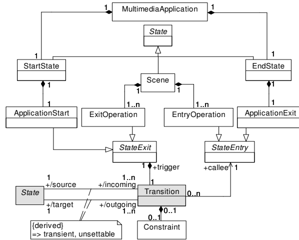
Fig. 9. Metamodel diagram for the temporal structure
