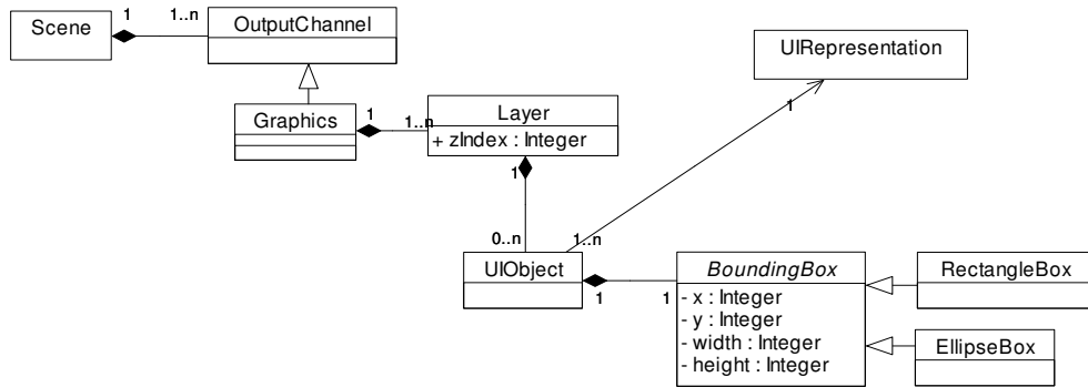
Fig. 6. Metamodel diagram for the user interface presentation
