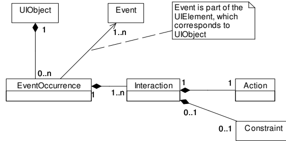
Fig. 7. Metamodel diagram for the interaction model
